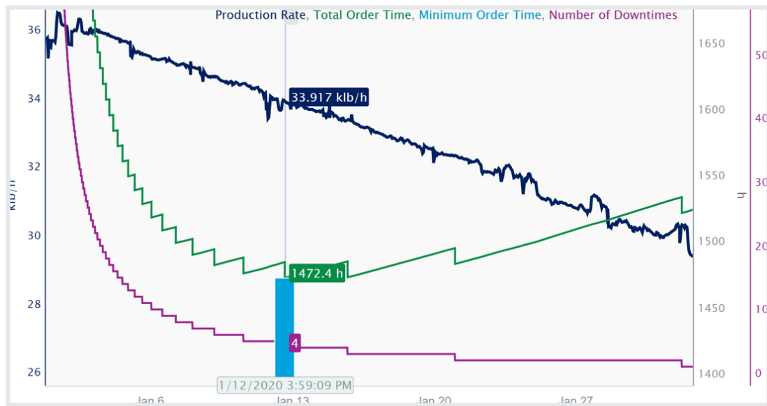
A screenshot of the Seeq Workbench showing the critical step of identifying the number of short maintenance shutdowns that optimizes total production run time.
